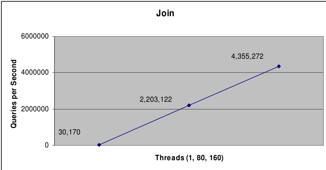
Chart 4 – JOIN performance of the eXtremeSQL ODBC API (queries/second).
