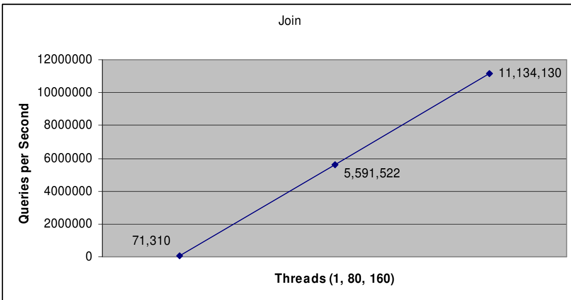
Chart 3 – JOIN performance of the eXtremeDB native API (queries/second).
