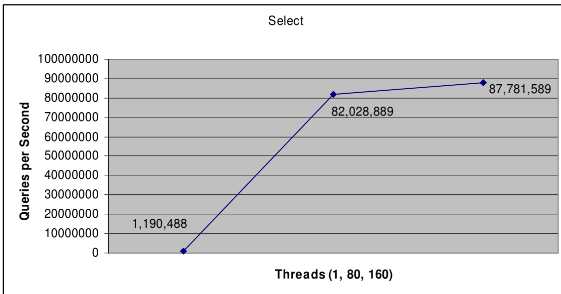
Chart 1 – SELECT performance of the eXtremeDB native API (queries/second).
