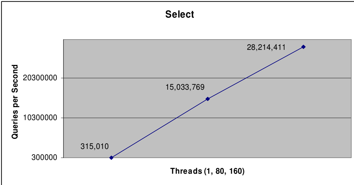
Chart 2 – SELECT performance of eXtremeSQL ODBC API (queries/second).
