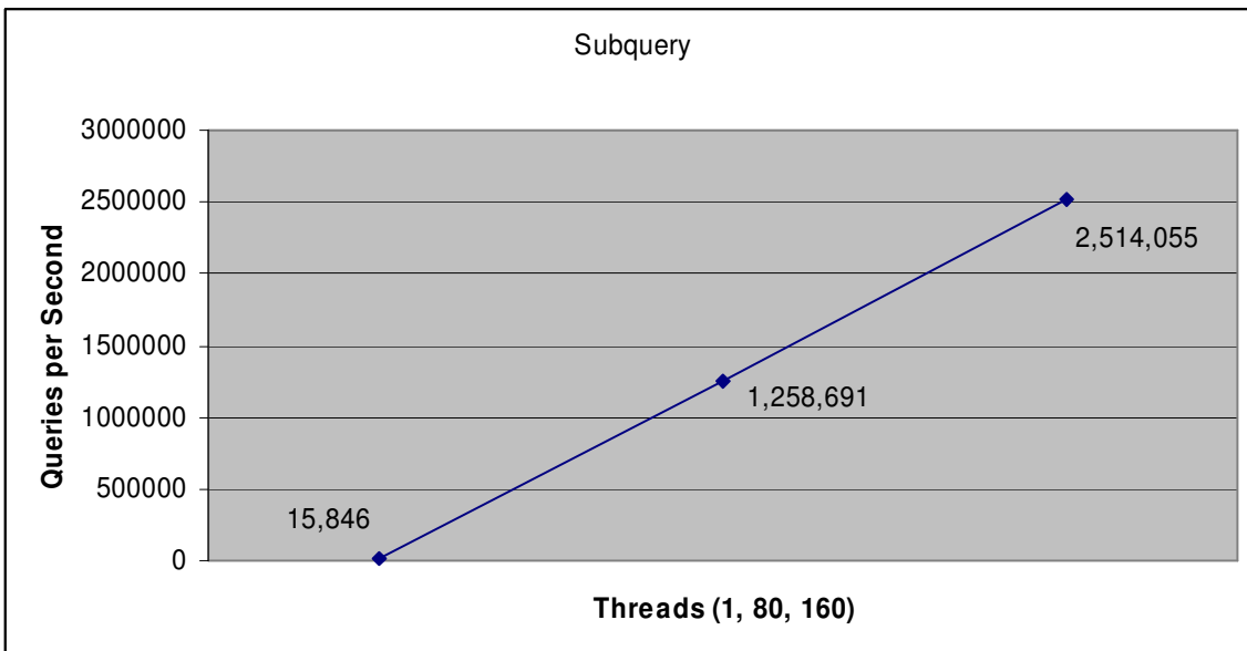
Chart 5 – SUBQUERY performance of the eXtremeDB native API (queries/second).
