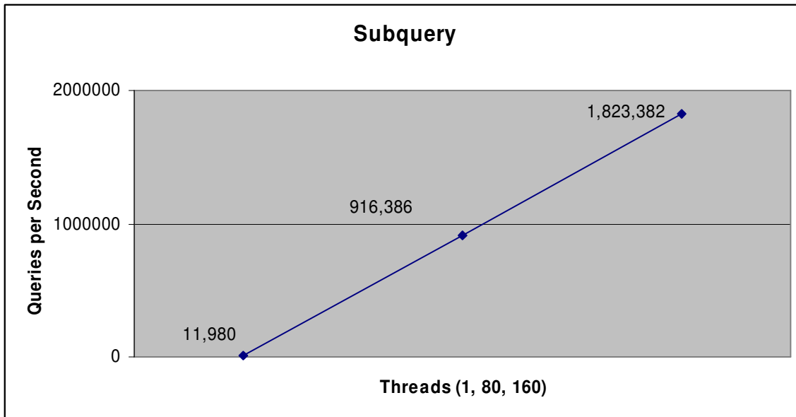
Chart 6 – SUBQUERY performance of the eXtremeSQL ODBC API (queries/second).
